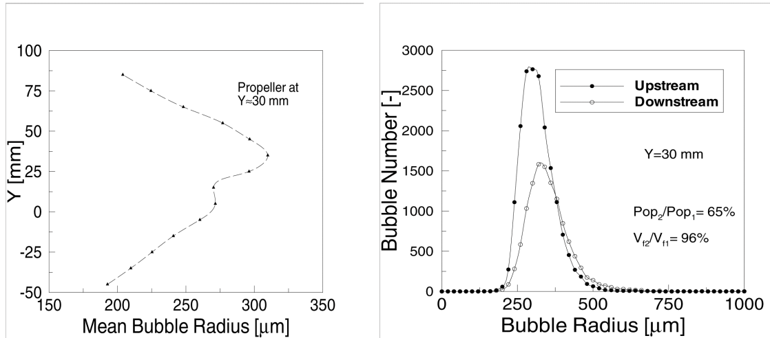
Fig 10. Left: bubble mean radius versus Y; right: size distribution upstream and downstream section Y=30 mm
