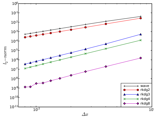
Figure 2: Log-log plot of l_2 -norms of solution as a function of \Delta x for the linear advection problem using the maximum allowable CFL number to set the time step for each of the numerical methods - the wave propagation, 2 nd , 3 rd , 4 th , and 8 th order RKDG. The slopes of the lines are tabulated in Table 1.
