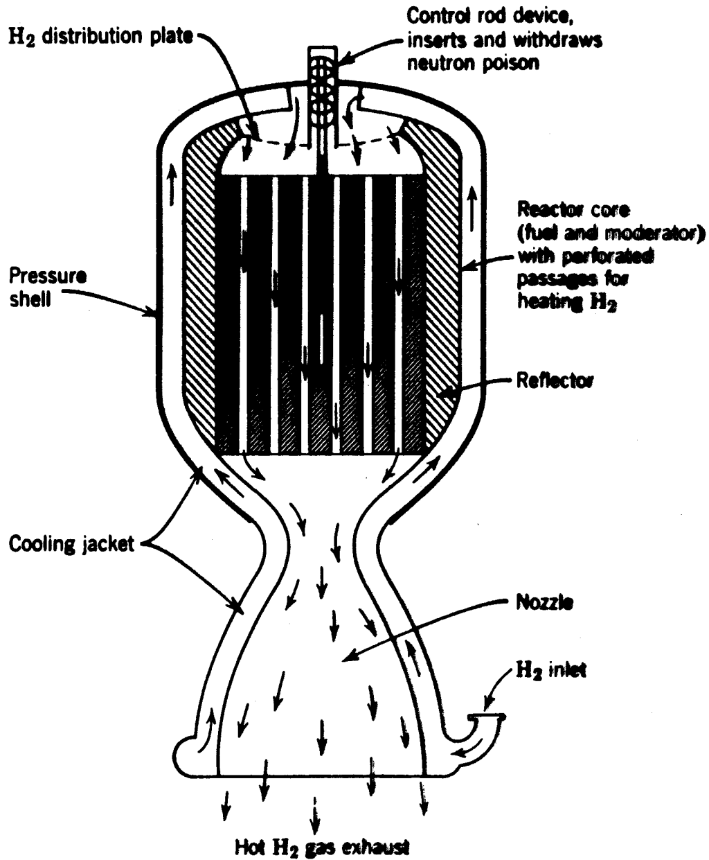
Fig. 14-6. Schematic diagram for fission reactor for nuclear rocket.
